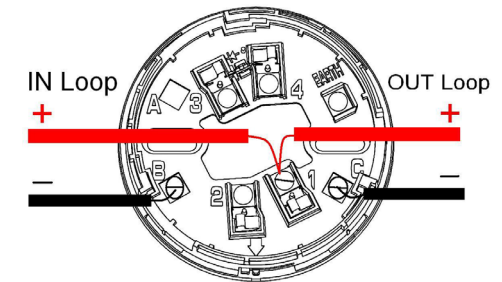
Isolator Base: Loop input terminals 1 & B Loop output terminals 1 & C
